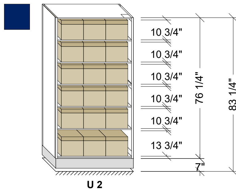
MOBILE 4-POST SHELVING 42"W x 16"D x 76 1/4"H
