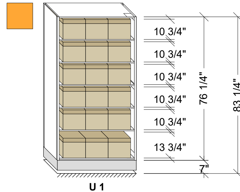
STATIC 4-POST SHELVING 42"W x 16"D x 76 1/4"H
